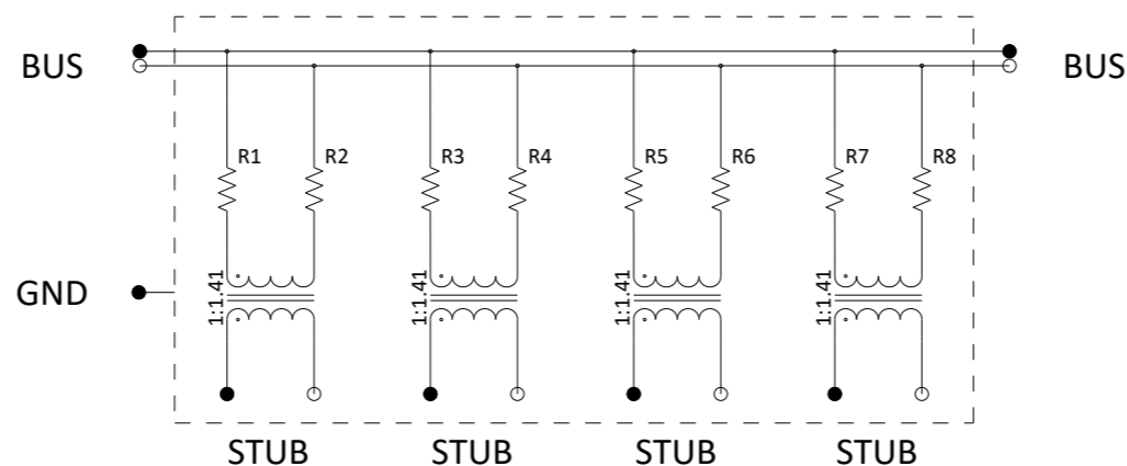
SCHMATIC DIAGRAM
